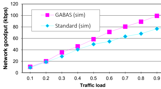
Fig. 2 The throughput networks against traffic load
