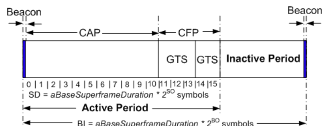
Fig. 1 an example superframe structure
