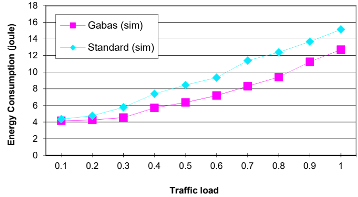
Fig. 4 The energy consumption against traffic load
